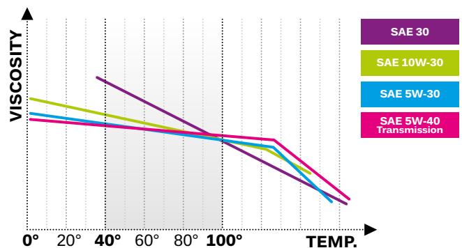
Viscosity performance
