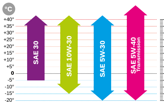
Temperature performance
